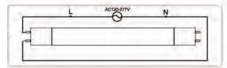
Single Ended Wiring Diagram
