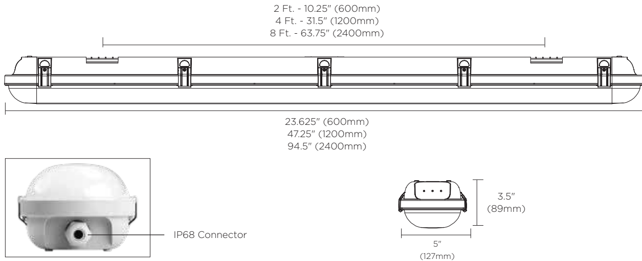
Surface installation
