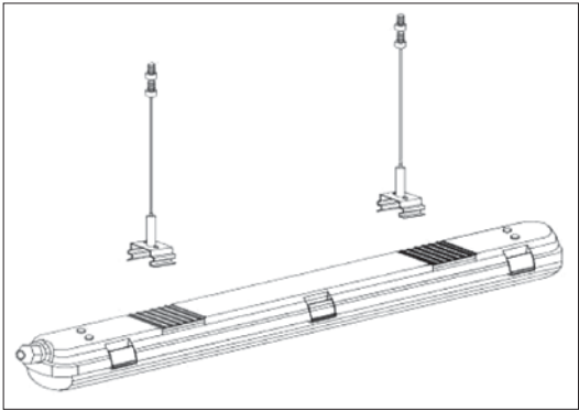
Suspension installation
