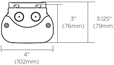
Suspension installation
